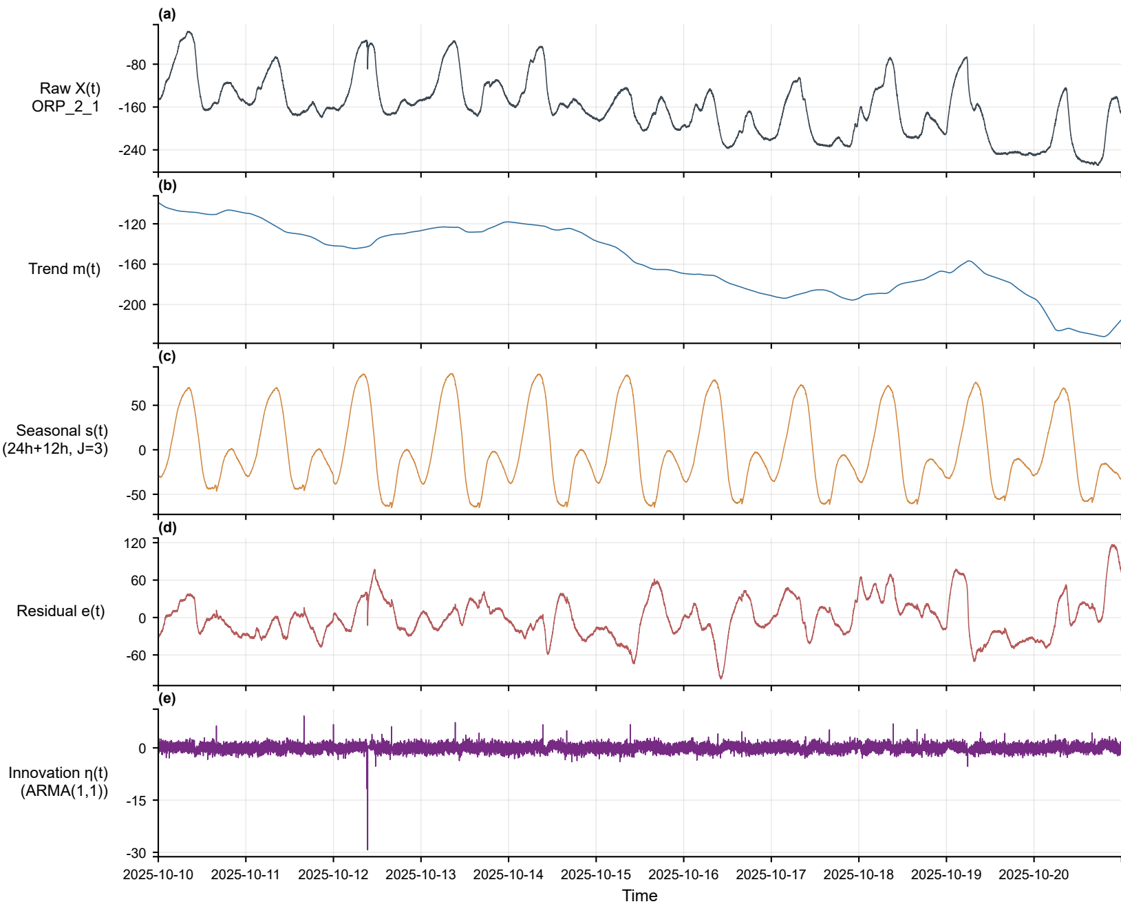
Multi-scale decomposition — ORP_2_1 (anaerobic, min) [2025-10-10~2025-10-20]
